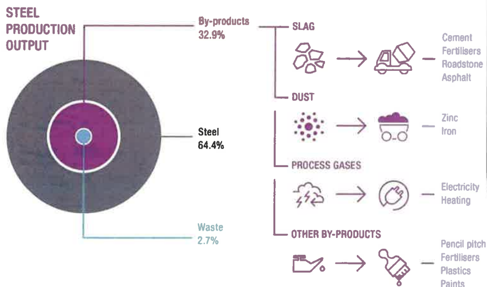
Main steelmaking by-products and their uses
